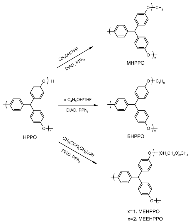
Scheme 2. Modifications of HPPO
